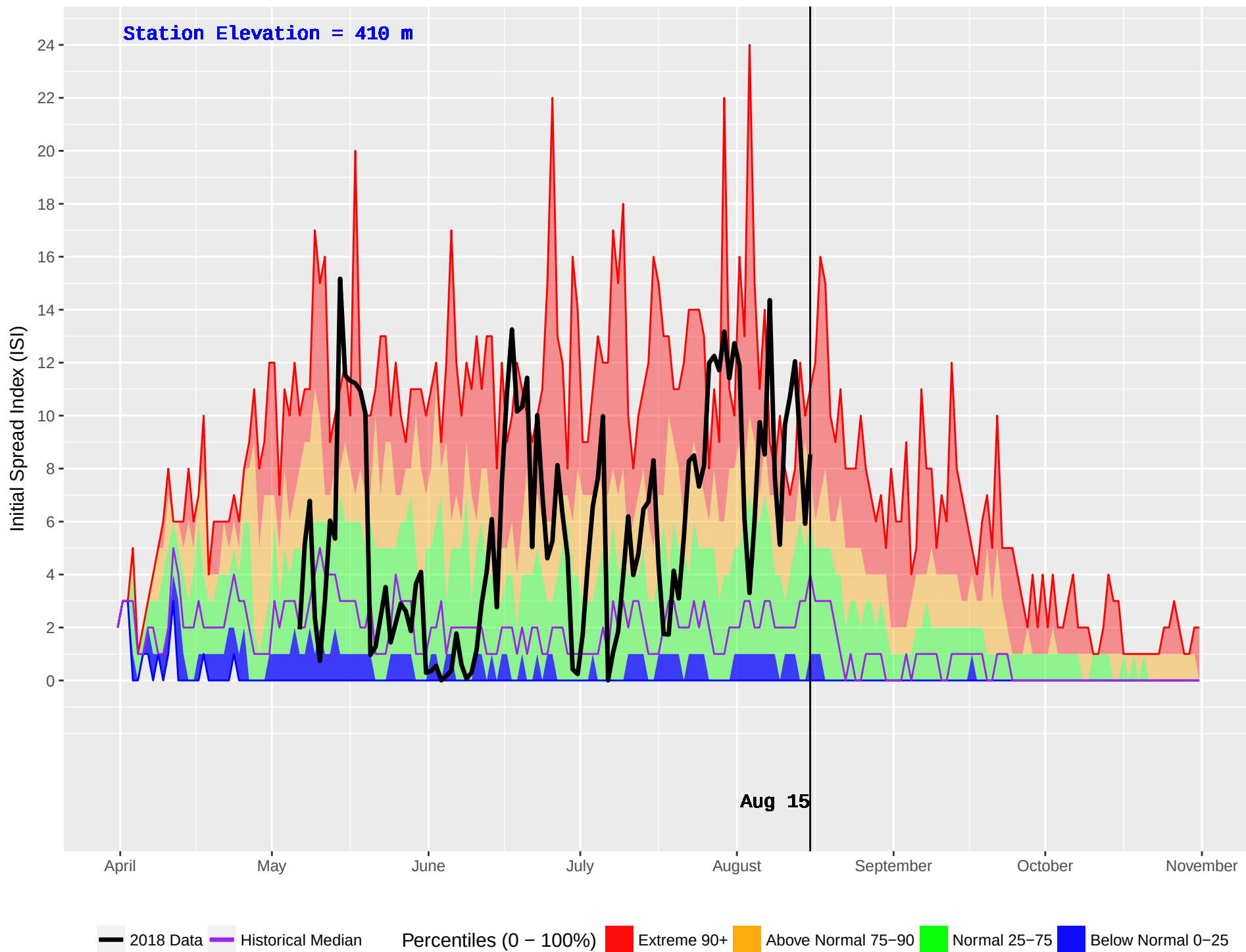
UPPER KISPIOX (431) : Historical (1986–2016) and Current (2018) Daily Initial Spread Index (ISI)
