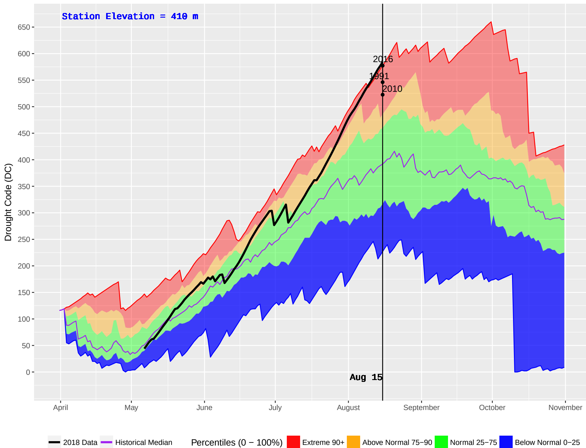
UPPER KISPIOX (431) : Historical (1986–2016) and Current (2018) Daily Drought Code (DC)
